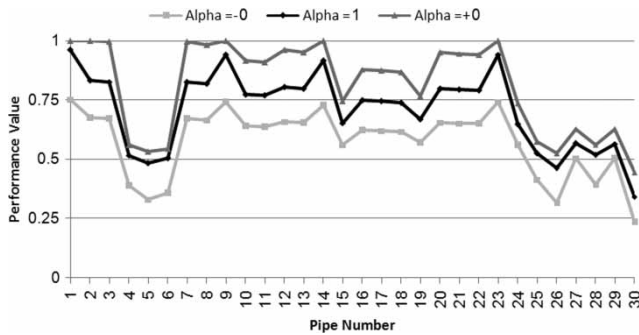
Figure 14 | Performance value of different pipes in terms of relative depth under maximum discharge ( Q_{\max} in 2035); \alpha -levels of 1 and 0 (– and + refer to lower and upper bounds, respectively).
