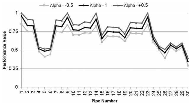
Figure 16 | Performance value of different pipes in terms of relative depth under maximum discharge ( Q_{\max} in 2035); \alpha -levels of 1 and 0.5 (– and + refer to lower and upper bounds, respectively).
