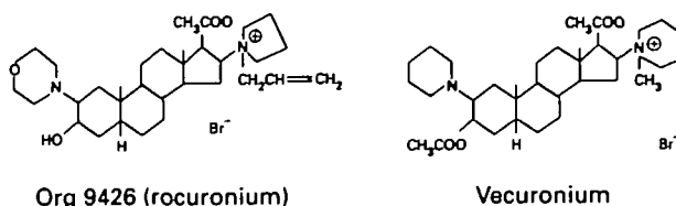
FIG. 1. Structural formulae of Org 9426 (rocuronium) and vecuronium.
