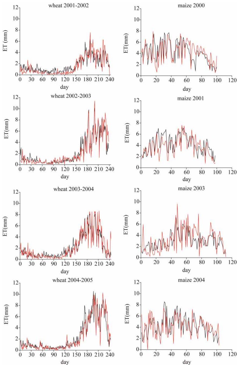
Figure 4 | The simulated and observed ET of winter wheat and summer maize.
