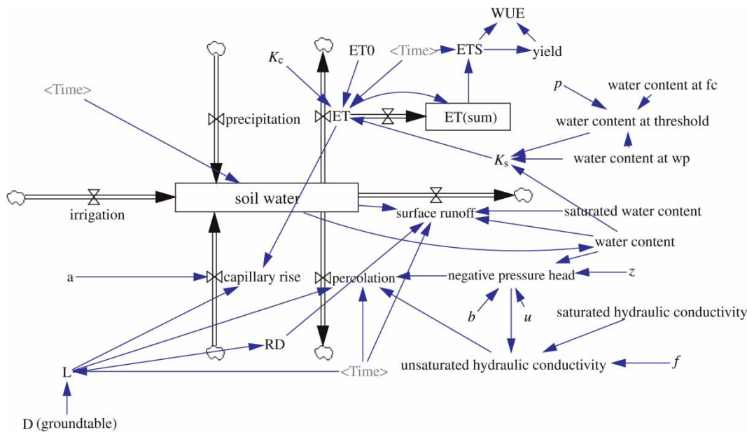
Figure 2 | The stock-flow structure of the dynamic soil water balance model. Note: ET(sum) and soil water are level variables; \Rightarrow is rate variable; \rightarrow is material flow or information chain; \oplus is source or leakage; others are auxiliary variable/constant variable/exogenous variable, and b, u, z, f are coefficients or parameters.
