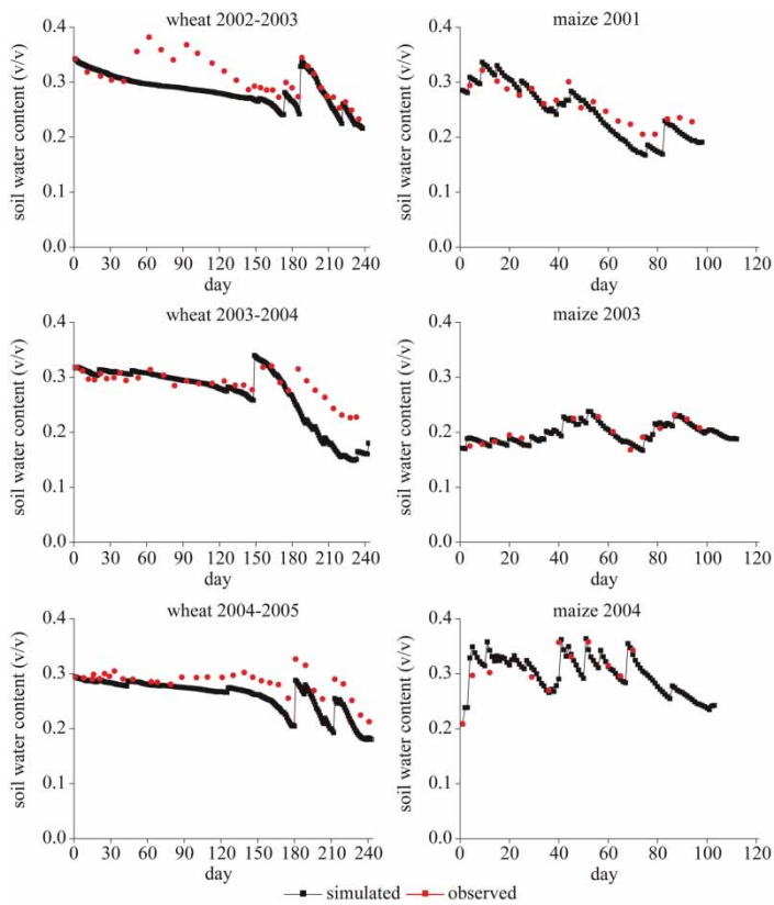
Figure 3 | Comparisons of the observed and simulated soil volumetric water content values of winter wheat and summer maize.
