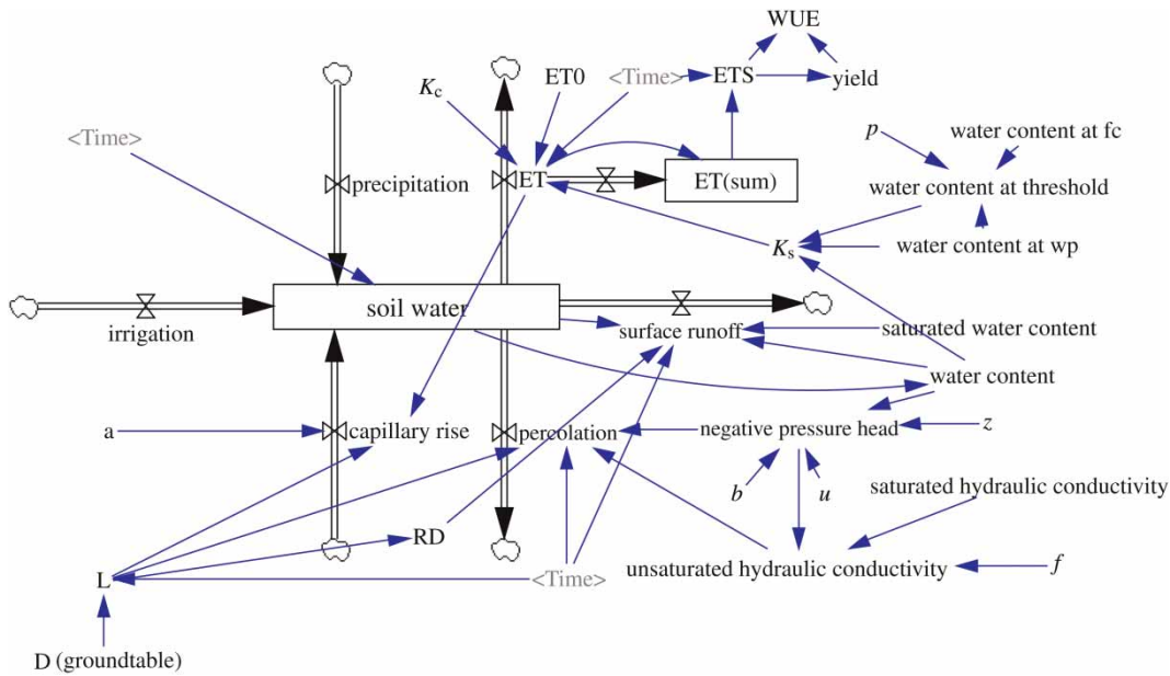
Figure 2 | The stock-flow structure of the dynamic soil water balance model. Note: ET(sum) and soil water are level variables; \rightleftarrows is rate variable; \longrightarrow is material flow or information chain; \oplus is source or leakage; others are auxiliary variable/constant variable/exogenous variable, and b, u, z, f are coefficients or parameters.
