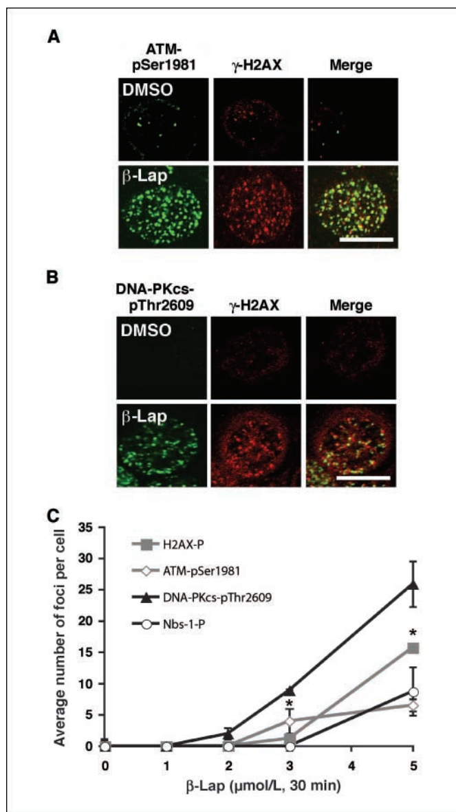
Figure 2. Dose-dependent ATM and DNA-PK activation after \beta -lap administration. MCF-7 cells were treated with 0 to 5 \mu mol/L \beta -lap for 30 min at which time samples were fixed and probed with antibodies to phosphorylated ATM at Ser1981 (ATM-pSer1981; A) or phosphorylated DNA-PKcs at Thr2609 (DNA-PKcs-pThr2609; B) and visualized by confocal microscopy. C, MCF-7 cells were treated with 0 to 5 \mu mol/L \beta -lap for 30 min; fixed; and probed for ATM-pSer1981, DNA-PKcs-pThr2609, and Nbs-1-p after 30 min. Quantitation of the average number of foci per cell per dose of \beta -lap-treated cells for \geq 60 cells per treatment. Points, means; bars, SE. Student's t test for paired samples, comparing Nbs-1-p or \gamma -H2AX foci per cell versus the number of DNA-PKcs-pThr2609 foci per cell at various doses of \beta -lap (*, P < 0.05 ). Bar, 20 \mu m.
