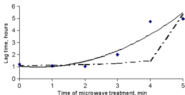
Figure 3 | Effect of microwave treatment time on lag time of E. faecalis growth. Broken line: theoretical curve produced using Equation (17); solid line: growth curve developed using Equation (18).
