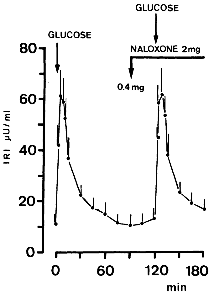
FIG. 2. Comparison of insulin responses to two consecutive intravenous glucose pulses (0.33 g/kg) given before and during an infusion of naloxone in normal subjects. No significant differences are observed between the two insulin responses. (Reproduced from ref. 38.)
