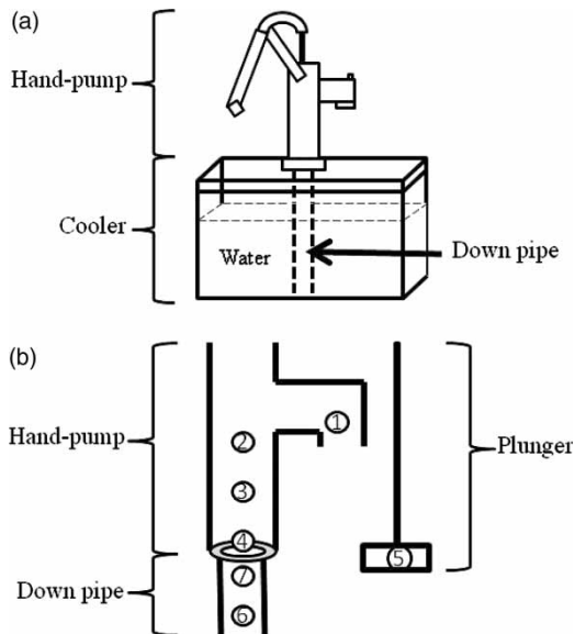
Figure 2 | (a) Schematic of laboratory hand-pump experiment; and (b) location of swabs (1–7) taken from the internal surface of the new hand-pump.
