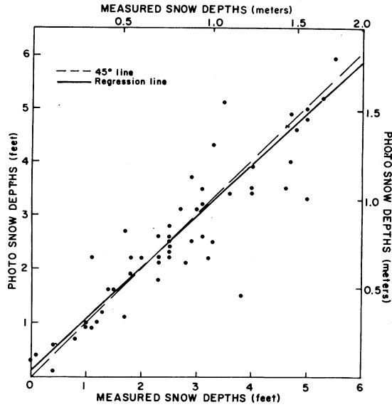
Fig. 2. Comparison of Photogrammetric and Measured Snow Depths for March 7, April 4, 1966 and March 12, March 26 and April 30, 1969.
