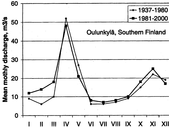
Fig. 1. Mean monthly discharges in Saukkoniva (measuring site: 68°55'N, 26°55'E, F = 5160 km 2 , L = 4.7%), Äyskoski (63°23'N, 26°40'E, F = 2157 km 2 , L = 17.9%), Muroleenkoski (61°51'N, 23°54'E, F = 6102 km 2 , L = 12.2%) and Oulunkylä (60°14'N, 24°59'E, 1680 km 2 , L = 2.5%). In southern and central Finland especially winter flow has increased during the observation period, in south-western Finland mean annual flow has also increased, and the date of the spring flood peak has shifted earlier. In the north, no trend in winter flow is observed.
