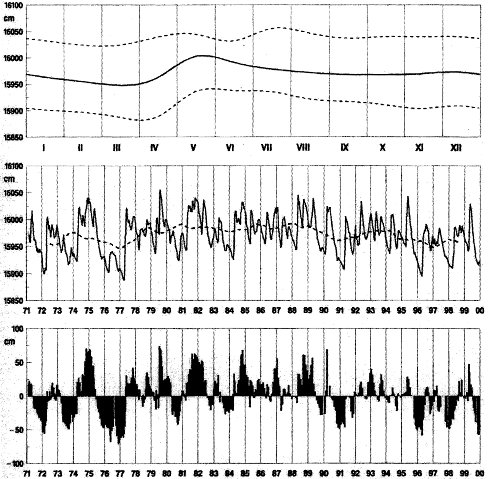
Fig. 3. Groundwater stage at Tullinkangas, southern Finland, 1971-1999. A: mean and extreme groundwater levels I-XII. B: annual variations and 3 year moving average of groundwater level. C: deviation from the mean level (Soveri et al. 2001).
