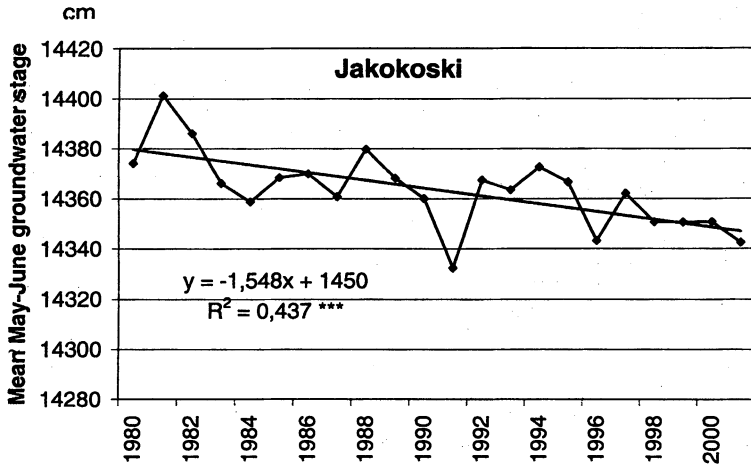
Fig. 4. May-June groundwater stage in 1980-2001 in Jakokoski, Northern Karelia (Mäkinen 2002)
