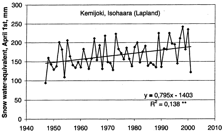
Fig. 5. Water equivalent of snow in some drainage basins in Lapland, northern Finland, central Finland and southern Finland on April 1st, 1947-2001.
