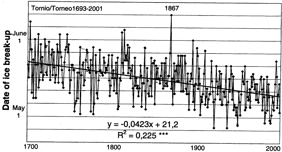
Fig. 7. Date of ice break-up in the lower reach of the river Tornionjoki (Tornio/Torneå) in the period 1693-2001 (Kajander 1995 and SYKE 2001). The Years of Great Famine in Finland culminated in 1867.
