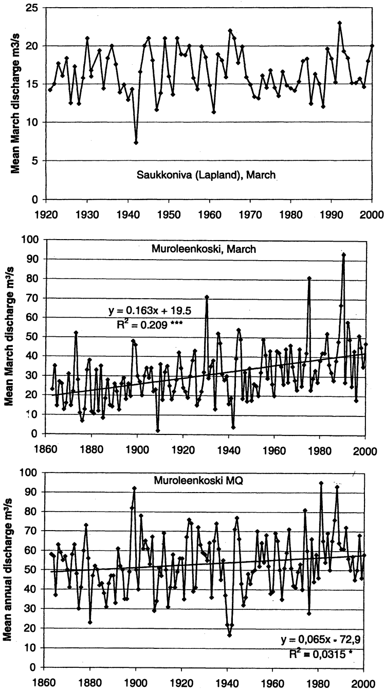
Fig. 2. Mean March discharge for Muroleenkoski and Saukkoniva as well as annual (MQ), annual maximum (HQ), July and November discharges for Muroleenkoski, compare with Fig. 1.
