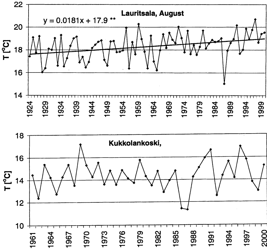
Fig. 6. Mean surface water temperature in August. Saimaa, Lauritsala (S-E Finland) 1924-2000 and Tornionjoki, Kukkolanoski (N-W Finland) 1961-2000 (Korhonen 2002).
