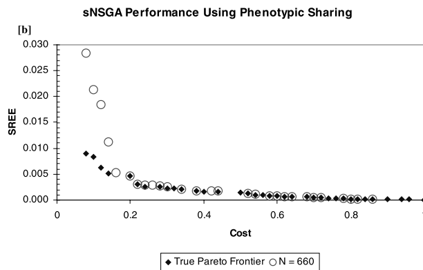
Figure 9 | sNSGA's performance relative to the true Pareto front using both (a) genotypic and (b) phenotypic sharing. The circles represent the best nondominated front attained in 40 generations.
