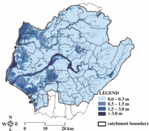
Figure 8 | Maximum inundation depths for 1-day maximum rainfall with 100-year under CIC-2.
