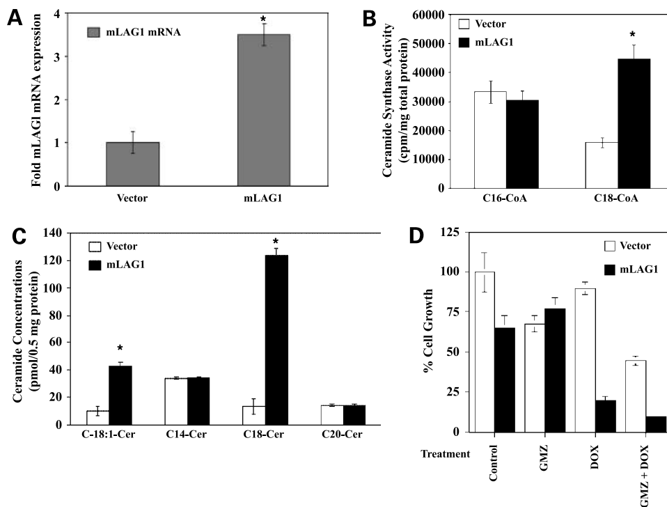
Figure 5. Roles of mLASS1/UOG1 expression on ceramide metabolism and gemcitabine/doxorubicin-induced growth inhibition in UM-SCC-22A cells. A , overexpression of mouse LASS1 in UM-SCC-22A cells were confirmed by Q-PCR as described in Materials and Methods. B , the effects of mouse LASS1 (mLASS1) on ceramide synthase activity for the generation of C_{18} -ceramide was confirmed by in vitro enzyme activity assay as described in Materials and Methods. C , the levels of endogenous ceramide in cells transfected with vector ( controls ) or with mLASS1 were measured by LC/MS. D , UM-SCC-22A cells were transfected with vector control or mLASS1 (for 36 h) before gemcitabine/doxorubicin treatments (48 h). After treatments, percent growth inhibition was determined by 3-(4,5-dimethylthiazol-2-yl)-2,5-diphenyltetrazolium bromide assays. The results represent at least three experiments, which were done in duplicates. Bars, SD. Statistical analysis was done as described in Materials and Methods. *, P < 0.05 , statistically significant.
