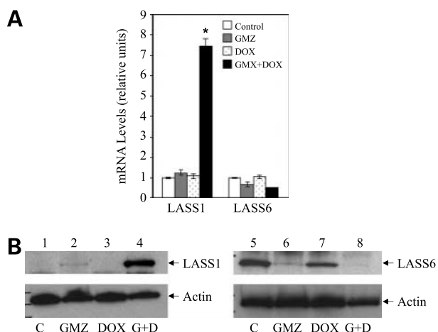
Figure 9. Modulation of mRNA expression levels of LASS genes and LASS1 and LASS6 protein levels in response to gemcitabine/doxorubicin-induced inhibition of tumor growth in UM-SCC-22A xenografts in vivo . A , mRNA levels of LASS1 and LASS6 were determined by Q-PCR as described in Materials and Methods. At least three experiments were done in triplicates; bars, SD. Statistical analysis was done as described in Materials and Methods. *, P < 0.05 , statistically significant. B , levels of LASS1 and LASS6 proteins of the extracted tumor tissues were determined by Western blotting. Actin levels are used as loading controls.
