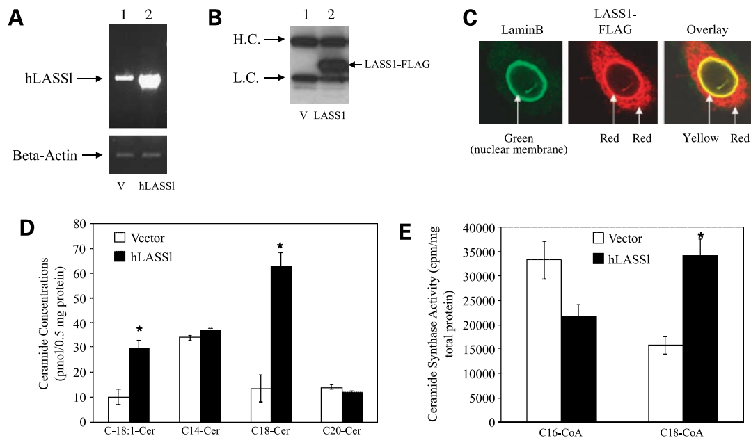
Figure 3. Induction of human LASS1 expression, which regulates ceramide synthase activity for the generation of C 18 -ceramide levels. A , overexpression of LASS1 (lane 2) was confirmed by RT-PCR, and compared with that of controls (lane 1) as described in Materials and Methods. B , partial purification of the FLAG-tagged protein by anti-FLAG antibody-conjugated agarose beads followed by Western blotting using the antibody against FLAG epitope as described in Materials and Methods. Vector (V)-transfected cells were used as control. L.C. and H.C., light-chain and heavy-chain peptides of the antibody used in immunoprecipitation. C , cellular localization of LASS1 was determined by immunofluorescence confocal microscopy using anti-FLAG and anti-LaminB antibodies as described in Materials and Methods. D , UM-SCC-22A cells were transfected with LASS1 for 48 h, and endogenous ceramide levels were measured by LC/MS. The ceramide levels were normalized to 0.5 mg total proteins. At least three experiments were done in duplicates; bars, SD. E , UM-SCC-22A cells were transfected with LASS1 for 48 h, and total microsomes were used to determine C 16 - and C 18 -ceramide synthase activity in vitro as described in Materials and Methods. Statistical analysis was done as described in Materials and Methods. *, P < 0.05 , statistically significant.
