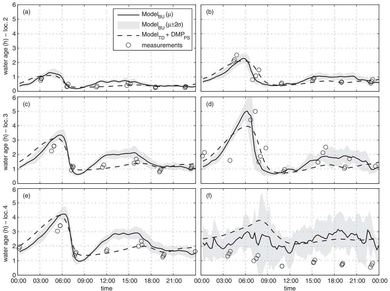
Figure 6 | Measured and modelled residence time (Model TD + DMP PS and Model BU ) in branched (a, c, e; scenarios 3 and 9) and looped (b, d, f; scenarios 4 and 10) network layout on locations 2 (a–b), 3 (c–d) and 4 (e–f) with a time scale of 15 min.
