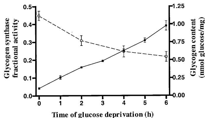
FIG. 1. Total glycogen content and GS activity in myoblasts cultured in the absence of glucose; effect of glucose readdition. Myoblasts were maintained for up to 6 h in DMEM Glu - . At the times indicated, total glycogen content of the cultures was determined (---, right y-axis). In the absence of glucose readdition, the GS activity was less, at every time point, than what was observed in nonstarved cultures. In separate cultures, DMEM Glu - was replaced with media containing 6.1 mmol/l glucose (Ham's F-10) for 15 min before extraction. The fractional activity of glycogen synthase was determined in these extracts (—, left y-axis). Results represent the mean \pm SE ( n = 7 ) in at least three subjects.
