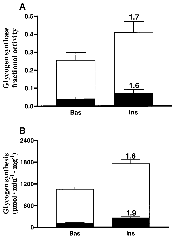
FIG. 3. Combined effects of insulin and glucose on GS activity and glycogen synthesis in cells cultured in the absence or presence of glucose. Cells were incubated in DMEM Glu - (□) or Ham's F-10 (6.1 mmol/l glucose) (■) for 5 h. Media were then replaced with Ham's F-10 containing 100 nmol/l insulin (Ins) for 15 min or not replaced (Bas) for 15 min and GS activity was determined (A); or media were replaced for 1 h and the rate of glycogen synthesis was determined (B). Results represent the mean ± SE ( n = 6) in at least three subjects. The insulin-mediated fold-activation over basal values is also indicated.
