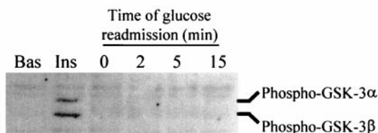
FIG. 6. Effects of insulin and glucose on GSK-3 activity and phosphorylation. Myoblasts were incubated in DMEM Glu - growth media for 5 h before replacement of media with Ham's F-10 (containing 6.1 mmol/l glucose) for the times indicated. Alternatively, cells were incubated in Ham's F-10 for 5 h before the addition of insulin (100 nmol/l) for the times indicated. Extracts were prepared and GSK-3 activity determined. Data are % of basal activity and mean \pm SE ( n = 6 ) in three subjects. Serine phosphorylation of GSK-3 \alpha and GSK-3 \beta was probed using phosphospecific antibodies in extracts from samples treated with 100 nmol/l insulin (Ins) or without 100 nmol/l insulin (Bas) for 15 min, or alternatively in myoblasts deprived of glucose for 5 h before readmission of Ham's F-10 for the times indicated. * P < 0.05 compared with basal values.
