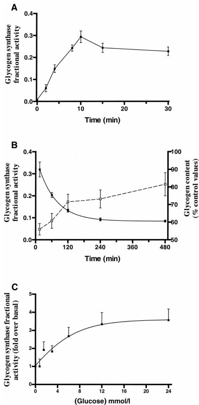
FIG. 2. Concentration- and time-dependent effects of glucose on GS activity in cells cultured in the absence of glucose. Myoblasts were incubated in DMEM Glu - growth media for 5 h before replacement of media with Ham's F-10 (containing 6.1 mmol/l glucose) for the times indicated (A and B). Total cellular glycogen content was also determined in cells after chronic refeeding (B) (----, right axis). Alternatively, myoblasts were incubated in DMEM Glu - growth media for 5 h before replacement of media with DMEM Glu - supplemented with different concentrations of glucose for 15 min (C). Extracts were prepared and the fractional activity of glycogen synthase determined. The resulting fractional activities represent the mean \pm SE ( n = 6 ) in at least three subjects.
