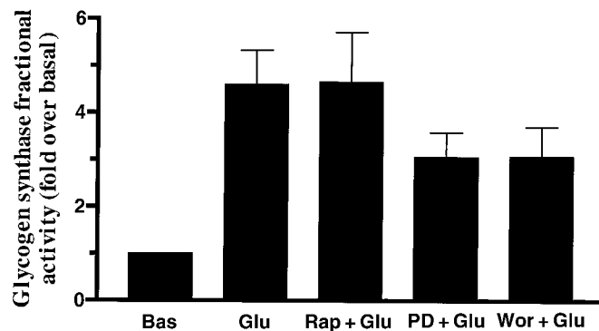
FIG. 5. Effect of selective inhibitors on activation of GS by glucose. Cells were maintained in DMEM Glu - for 5 h before further incubation for 15 min in DMEM Glu - (Bas) or DMEM growth media supplemented with 5.5 mmol/l glucose. Alternatively, cells were treated with 100 nmol/l rapamycin (Rap) for 15 min, 50 μmol/l PD98059 (PD) for 1 h, or 100 nmol/l wortmannin (Wor) for 15 min before the addition of glucose (Glu). Extracts were prepared and the activity of GS determined. Results are expressed as the fold-activity over basal (Bas) and represent the mean ± SE ( n = 3) in three subjects.
