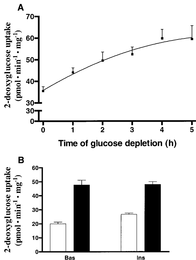
FIG. 4. 2-Deoxyglucose uptake in cells preincubated in the absence of glucose. Cells were maintained in DMEM Glu - growth media for up to 5 h. At the times indicated, the rate of glucose uptake was determined (A). Alternatively, cells were maintained in DMEM Glu - (□) or Ham's F-10 (6.1 mmol/l glucose) (■) for 5 h before the addition of 100 nmol/l insulin (Ins) or not adding insulin (Bas) for 15 min and the rate of glucose uptake determined (B). Results represent the mean ± SE ( n = 8) in three subjects.
