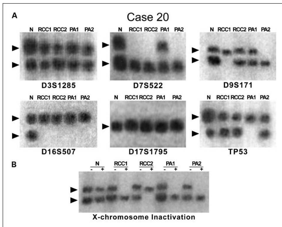
Fig. 2. Representative results (Case 20) of LOH analysis (A) and X-chromosome inactivation analysis (B). A, DNA was prepared from normal tissue and from multiple separate papillary tumors, amplified by PCR using polymorphic markers D3S1285, D7S522, D9S171, D16S507, D17S1795, and TP53, and separated by gel electrophoresis. B, cells from separate papillary tumors show different patterns of X-chromosome inactivation, consistent with independent origin. Arrows, allelic bands; N, normal tissue (control); RCC, renal cell carcinoma; PA, papillary adenoma; +, after Hha I endonuclease digestion; -, without Hha I endonuclease digestion (control).
