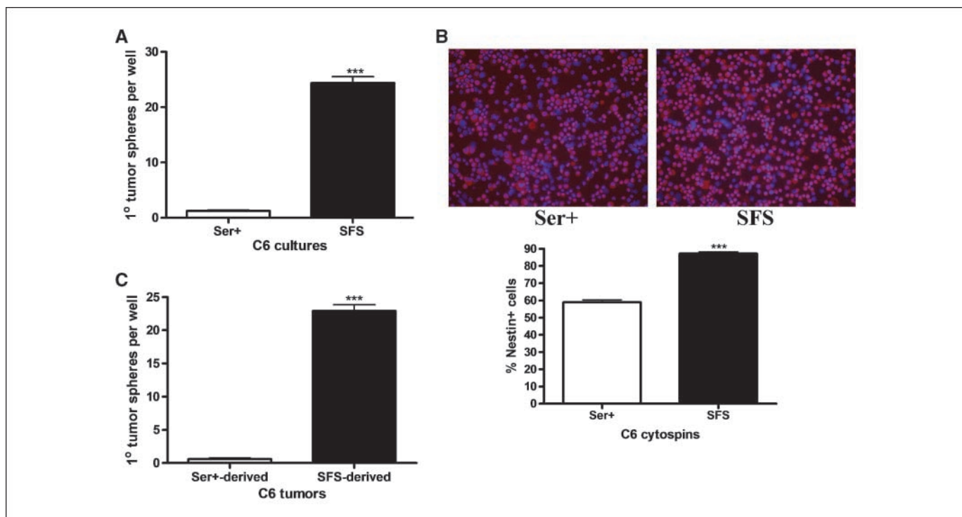
Figure 1. Relative CSC content in C6 Ser+ and SFS cultures and tumors. A , tumor sphere-forming assay: 100 cells plated per well. B , cytopins of C6 cultures stained for nestin (Texas red; red). Nuclei stained with 4',6-diamidino-2-phenylindole (blue), \times 200 . Histogram: image analysis of nestin staining. Eight fields analyzed per group. Cells displaying Texas red fluorescence above background (established using Texas red-conjugated IgG control) were counted as nestin-positive. C , ex-vivo tumor sphere-forming assay using established tumors (4 wk post-implantation).
