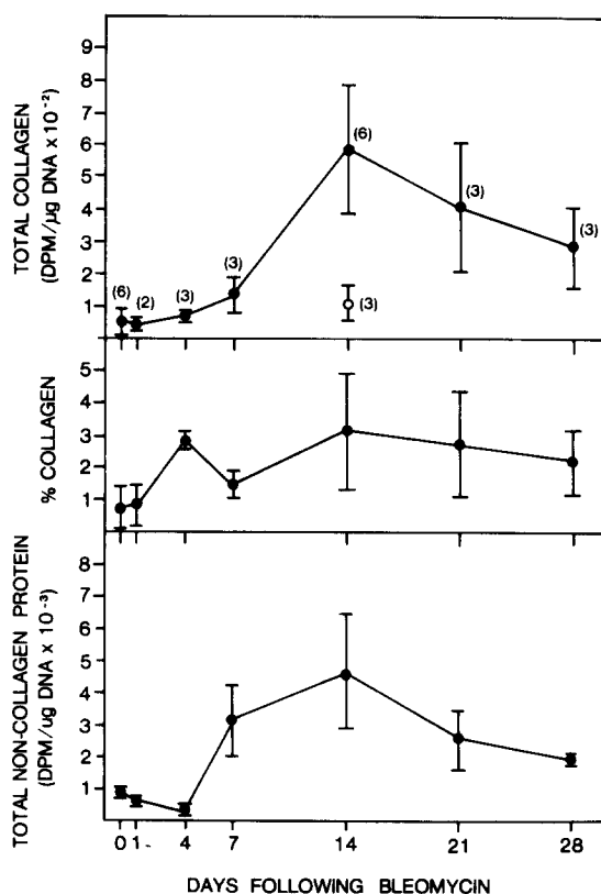
FIGURE 2. [ ^3 H]Proline incorporation into collagen and noncollagen protein of lung fibroblasts recovered from bleomycin-treated animals. At sequential time points ( \bullet ) after intratracheal bleomycin instillation, progressively increasing [ ^3 H]proline incorporation into both collagen ( upper panel ) and noncollagen protein ( lower panel ) was observed. Peak [ ^3 H]proline incorporation occurred at 14 d after bleomycin. Collagen synthesis decreased after 14 d but remained above baseline to 28 d. The proportion of [ ^3 H]proline incorporated into collagen remained two- to threefold higher than background ( middle panel ). Total collagen synthesis in rats 14 d after intratracheal injection with saline ( \circ ) instead of bleomycin was not different from untreated controls ( upper panel ). The number of animals in each group is indicated in brackets in the upper panel.
