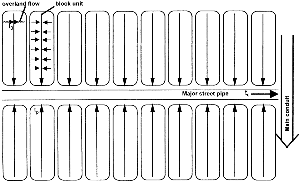
Fig. 3. Complex urban basin with drainage from a sub-basin into a main sewer. The sub-basin, for which the kinematic travel time of the major street pipe is t_c , consists of 20 identical street block drainage units with overland flow of concentration time t_o and pipe flow of concentration time t_p .
