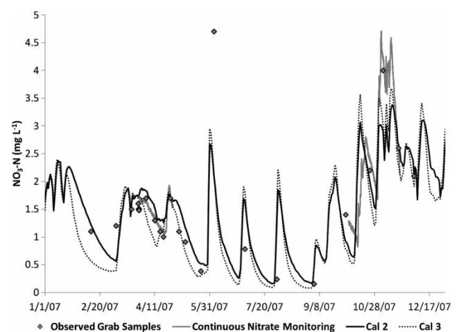
Figure 7 | INCA-N simulated \text{NO}_3\text{-N} concentrations from Calibration 2 and Calibration 3 compared to grab samples and continuous automatic monitoring for the Yläneenjoki catchment in 2007.
