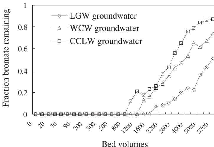
Figure 3 Effect of source water on \text{BrO}_3^- removal. (YUB carbon, influent \text{BrO}_3^- = 100 \mu\text{g/L} , EBCT = 8 min)
