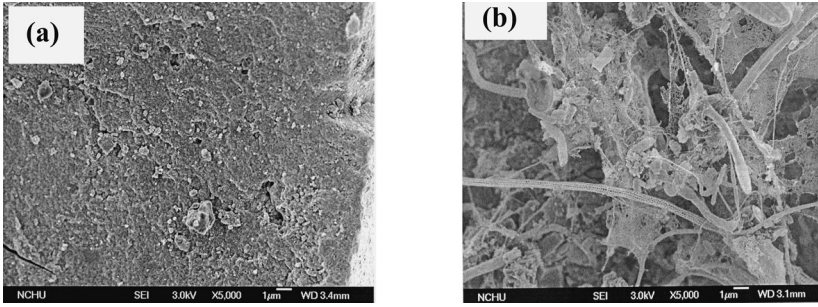
Figure 5 SEM micrograph of GAC surface (a) new GAC, (b) GAC after 9 months
