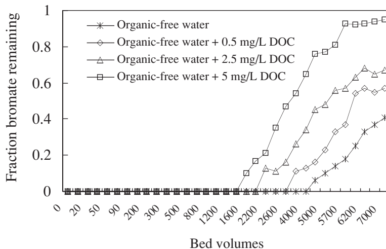
Figure 2 Effect of DOC on \text{BrO}_3^- removal. (YUB carbon, influent \text{BrO}_3^- = 100 \mu\text{g/L} , EBCT = 8 min)
