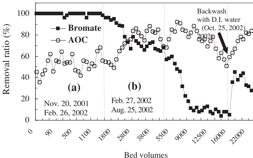
Figure 6 AOC and \text{BrO}_3^- removal in GAC filter during period (a) influent AOC = 124–187 \mu\text{g} acetate-C/L, \text{BrO}_3^- = 18–47 \mu\text{g} /L, (b) influent AOC = 91–226 \mu\text{g} acetate-C/L, \text{BrO}_3^- = 87–163 \mu\text{g} /L
