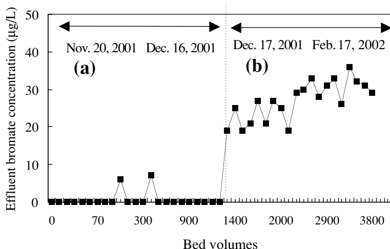
Figure 4 \text{BrO}_3^- removal in GAC filters during period (a) influent \text{BrO}_3^- = 18\text{--}47 \mu\text{g/L} , (b) influent \text{BrO}_3^- = 94\text{--}163 \mu\text{g/L}
