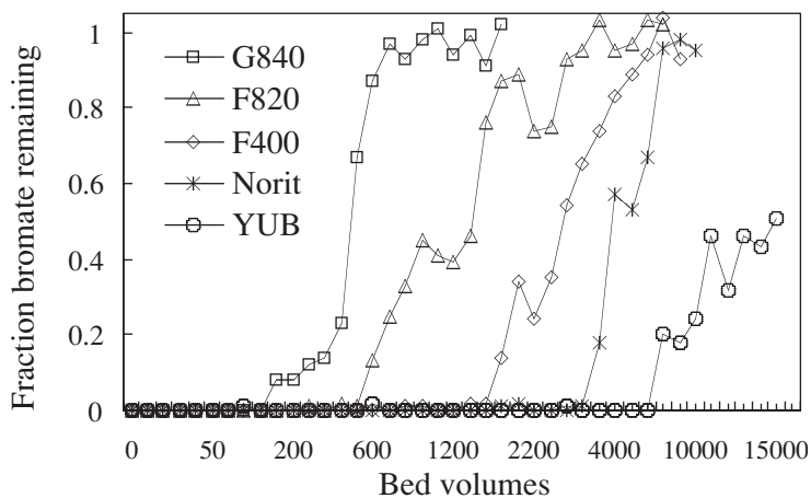
Figure 1 Effect of GAC types on \text{BrO}_3^- removal (influent \text{BrO}_3^- = 100 \mu\text{g/L} , EBCT = 8 min)
