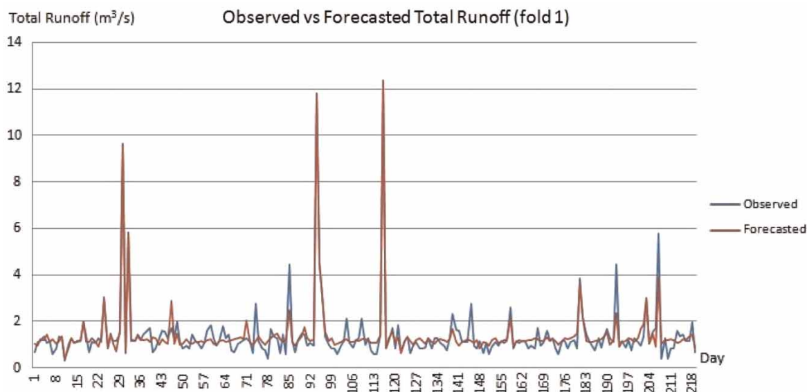
Figure 4 | Comparison of forecasted versus observed total runoff using the best testing WA-ANN model (Fold 1).
