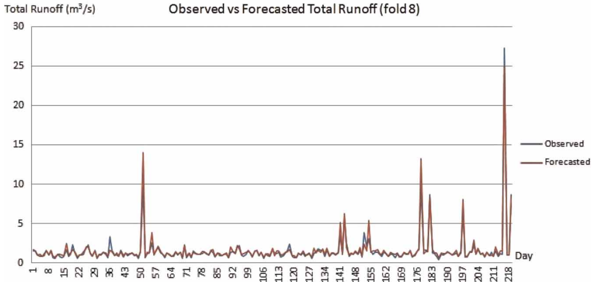
Figure 2 | Comparison of forecasted versus observed total runoff using the best testing MARS model (Fold 8).
