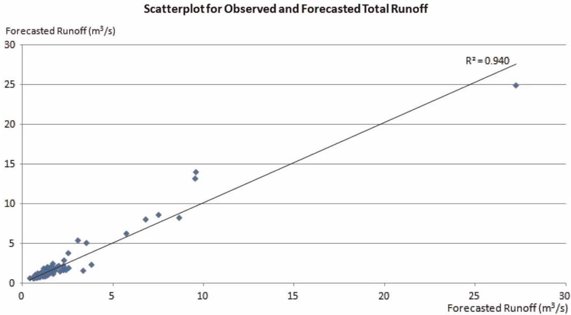
Figure 5 | Scatterplot comparing observed and forecasted total runoff using the best testing MARS model (Fold 8).
