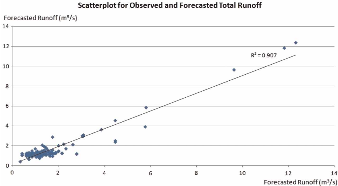
Figure 7 | Scatterplot comparing observed and forecasted total runoff using the best testing WA-ANN model (Fold 1).
