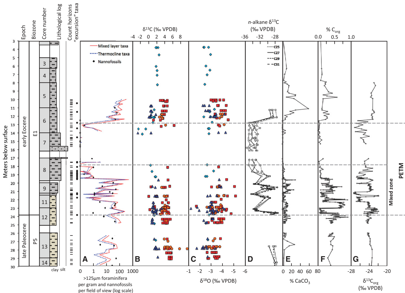
Figure 1. Stratigraphic log of Tanzania Drilling Project Site 14 (TDP-14) with geochemical and biotic records of the Paleocene–Eocene Thermal Maximum (PETM). Log records epoch, planktonic foraminiferal biozone (Berggren and Pearson, 2005), lithological variation (dashed gray is clay and silty clay, dotted gray is fine-grained sandstone), horizons sampled for assemblage analysis (dashes), and horizons containing “excursion taxa” (black circles). A: Assemblage data of mixed layer (red)– and thermocline (blue)–dwelling planktonic foraminifera and calcareous nannofossils (black diamonds) on a log scale from TDP-14B. B: Planktonic foraminifera \delta^{13}\text{C} from single specimens of the mixed-layer genera Morozovella (red squares) and Acarinina (orange circles) and thermocline genus Subbotina (light blue diamonds); also included are the multiple-specimen Subbotina data (blue triangles) from Handley et al. (2008) from TDP-14B (VPDB–Vienna Peedee belemnite). C: Planktonic foraminifera \delta^{18}\text{O} (symbols as in B). D: n -alkane \delta^{13}\text{C} data from TDP-14A (Handley et al., 2008) (open squares) and new data from this study between ~20 m and 24 m (gray circles). E: Bulk sediment weight percent \text{CaCO}_3 . F: Bulk sediment weight percent organic carbon. G: Bulk sediment \delta^{13}\text{C} of organic carbon. Gray dashed lines at 24 m to ~13 m denote PETM interval, with mixed interval highlighted between 24 m and ~18 m. For further details of lithology of TDP-14, see Handley et al. (2012).
