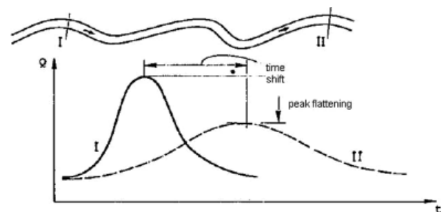
Figure 1 | Propagation and deformation of a hydrograph between two sections of the river.
