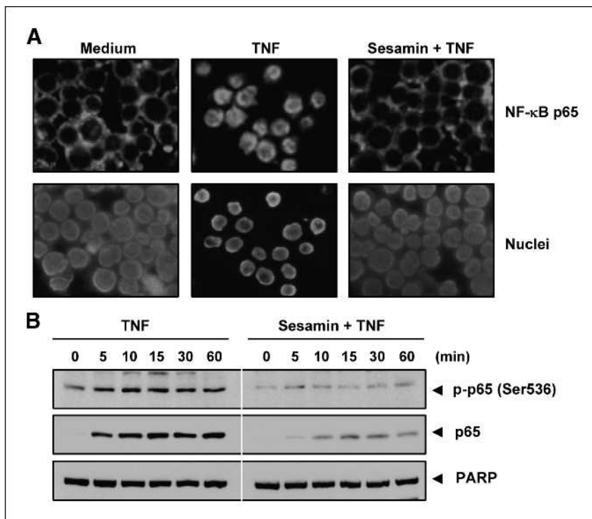
FIGURE 5. A, sesamin inhibits the TNF-induced nuclear translocation of p65 assayed by immunocytochemical analysis. KBM-5 cells were initially treated with 100 \mu M sesamin for 12 h and then exposed to 0.1 nmol/L TNF for 15 min. After cytospin, immunocytochemical analysis was done as described under Materials and Methods. B, sesamin inhibits the TNF-induced phosphorylation of p65. KBM-5 cells were either nontreated or pretreated with 100 \mu M sesamin for 12 h and then treated with 0.1 nmol/L TNF for the indicated times. Nuclear extracts were prepared and analyzed by Western blotting using p65 and phospho-specific p65 antibodies. For loading control of nuclear extracts, the membrane was reblotted with anti-poly ADP ribose polymerase (PARP) antibody, respectively.
