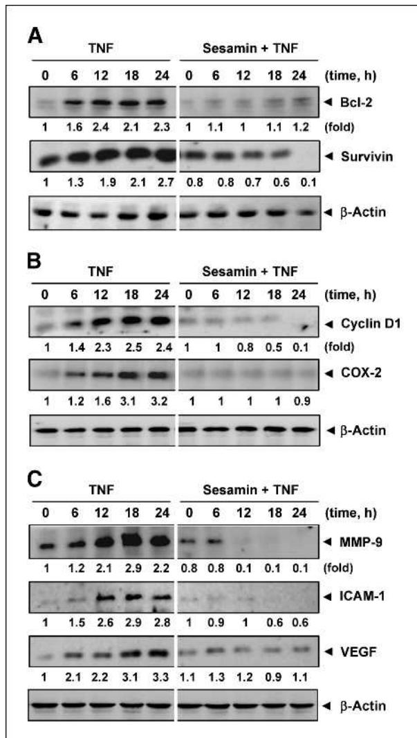
FIGURE 2. A, sesamin suppresses the expression of TNF-induced tumor cell survival proteins. KBM-5 cells were incubated with 100 \mu M sesamin for 12 h and then treated with 1 nmol/L TNF for the indicated times. Whole-cell extracts were prepared and analyzed by Western blotting using the indicated antibodies. B and C, sesamin inhibits the expression of tumor cell-proliferative and metastatic proteins. KBM-5 cells were incubated with 100 \mu M sesamin for 12 h and then treated with 1 nmol/L TNF for the indicated times. Whole-cell extracts were prepared and analyzed by Western blotting using the indicated antibodies. Anti- \beta -actin antibody was used as a loading control. Densitometric values of bands were corrected based on \beta -actin and were expressed relative to that of nontreated cells, which was set as 1.0.
