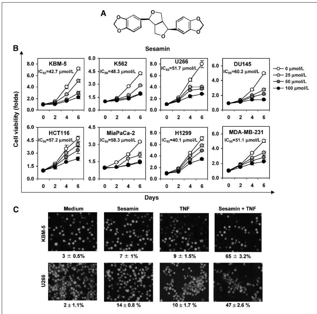
FIGURE 1. A, chemical structure of sesamin. B, sesamin suppresses tumor cell proliferation. Cells were incubated with 0, 25, 50, and 100 μmol/L sesamin for different days. Cell proliferation was then analyzed by the MTT method as described under Materials and Methods. C, sesamin potentiates TNF-induced cytotoxicity. KBM-5 ( 1 \times 10^5 ) or U266 ( 1 \times 10^5 ) cells were incubated with 100 μmol/L sesamin for 12 h and then incubated with 1 nmol/L TNF for 24 h. The cells were stained with a Live/Dead assay reagent for 30 min and then analyzed under a fluorescence microscope as described under Materials and Methods.
