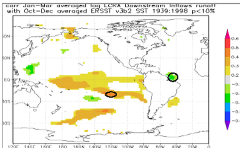
Figure 6 | Correlation map of winter downstream flows with fall sea surface temperatures. Circled regions indicate strong positive and negative correlations used to derive the ERSST3 index.
