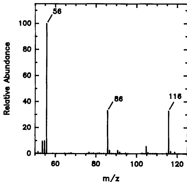
Figure 6. Mass spectrum of nitrosomorpholine generated from the oxidation of hydroxyurea in the presence of morpholine. Oxidation of hydroxyurea (0.3 mM) with 10 \mu\text{M} \text{CuSO}_4 and 2 mM \text{H}_2\text{O}_2 was carried out in the presence of 10 mM morpholine to trap generated NO. The reaction mixture was extracted with dichloroethane, concentrated under \text{N}_2 , and analyzed by GC/MS. A peak eluting at 3.8 min showed a molecular ion of m/z 116 and base fragment ion of m/z 56.
