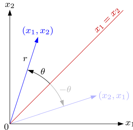
Fig. 2. Polar coordinates (r, \theta) in the (x_1, x_2) -space. The red line represents the set of two-body coincidence points.
