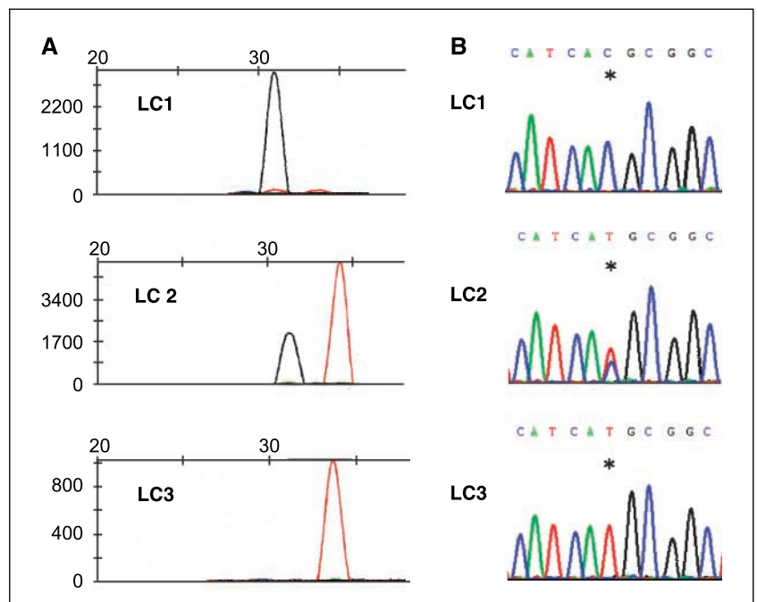
Figure 2. Representative examples of the mutant-enriched PCR assay. A , chromatogram of second letter in codon 790 determined by a single-base primer extension assay after enrichment of mutant alleles. Black and red peaks, C (wild-type nucleotide) and T (mutant-type nucleotide), respectively. Only wild-type sequence (C) was detected in LC1. Both wild-type (C) and mutant (T) sequences were detected in LC2. Only mutant sequence (T) was detected in LC3. B , corresponding sequence chromatograms for the product of the mutant-enriched PCR assay.
