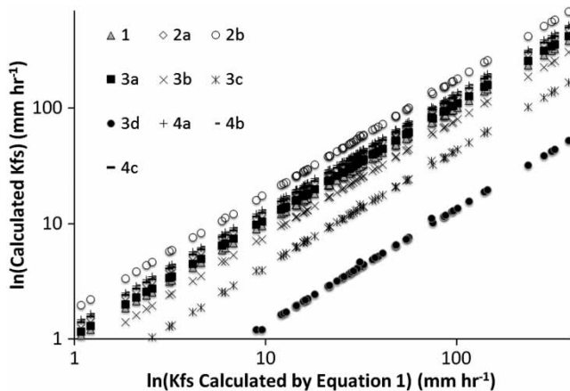
Figure 3 | Comparison of logarithmic Kfs values calculated using different formulae described in Table 2 against the Glover solution (Equation (1)), shown as 1:1 line. The number of data points was reduced to provide more clarity to the graphs.
