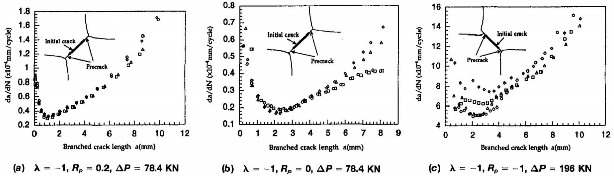
Fig. 1 Crack growth rates together with crack paths
