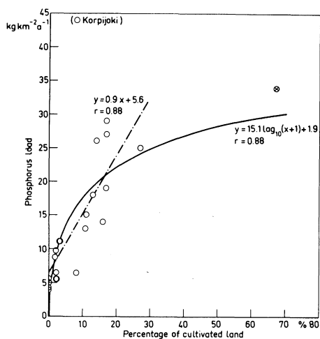
Fig. 3. Dependence of the diffuse phosphorus load on the percentage of cultivated land in the basin. — Value \circ included. - - - Value \circ excluded.
