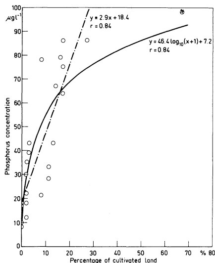
Fig. 2. Dependence of the total phosphorus concentration on the percentage of cultivated land in the basin. — Value \circ included. - - - Value \circ excluded.
