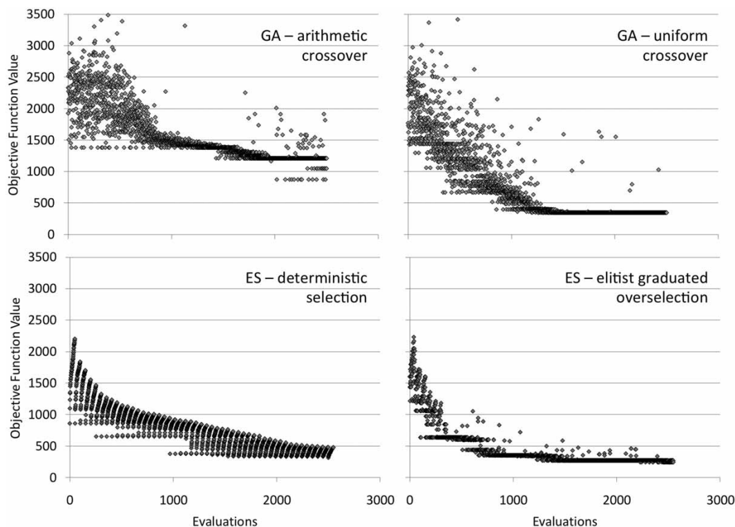
Figure 5 | Convergence of four algorithms, shown for the best trial for each algorithm.
