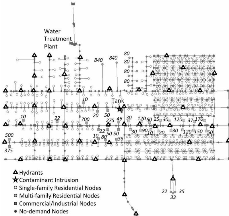
Figure 2 | Micropolis network and location of consumers. Labels indicate maximum population over a 24-hour time period at commercial/industrial nodes and multi-family residential nodes. Single-family residential nodes are initialized with 1–6 consumers at each node.
