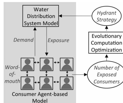
Figure 1 | Flowchart representing the simulation–optimization approach. The grey box encloses the ABM framework that couples agent simulation with a water distribution system model.
