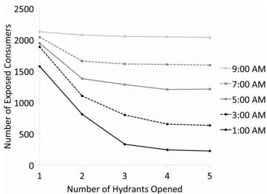
Figure 8 | Sensitivity analysis of performance of opening sub-sets of hydrants. Results are shown for the best solution for each response time (solutions shown in Figure 7). Number of exposed consumers (y-axis) is the average of 30 realizations of each strategy.
