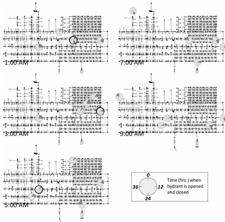
Figure 7 | Hydrant opening strategy corresponding to the best solution for different delays. Bold hydrant indicates the decision that appears in all solutions for response times of 1:00, 3:00, and 5:00 a.m.
