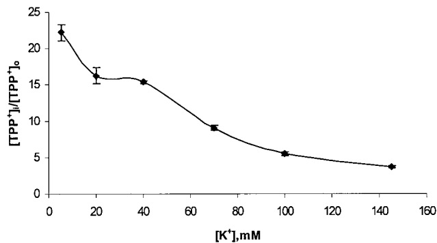
FIGURE 2. Effect of K^+ concentration in the medium on TPP^+ accumulation in rat lenses. Rat lenses were incubated in the presence of 10 \mu M TPP^+ for 18 hours, and TPP^+ uptake was measured as described in the Materials and Methods section. Data are presented as means \pm SE ( n \geq 4 ).
