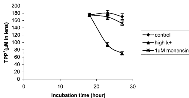
FIGURE 5. TPP + efflux from lenses. After an 18-hour incubation in the TC-199 medium with 10 \mu M TPP + , 1 \mu M monensin was added into the media. One group of the lenses was transferred to high-K + medium with 10 \mu M TPP + . [ 3 H]TPP + was measured after an additional 5- or 9-hour incubation. Data are presented as means \pm SE ( n \geq 4 ).
