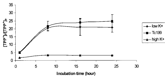
FIGURE 1. Accumulation of TPP + in rat lenses incubated in low-K + or high-K + balanced salt solution and modified TC-199 medium. TPP + (10 μM) was added to the medium, and the lenses were harvested as described in the Materials and Methods section. TPP + in was calculated assuming water content of 62% of wet weight in the lens. Data are presented as means ± SE for a representative experiment in which each group contained at least four lenses. The entire experiment was repeated at least twice.
