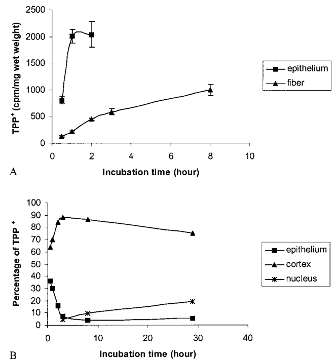
FIGURE 3. (A) TPP^+ accumulation in lens capsules and fibers. Rat lenses were incubated in TC-199 medium with 10 \mu M TPP^+ and were dissected at different time points. The TPP^+ uptake was measured as described in the Materials and Methods section. Data are presented as means \pm SE ( n \geq 4 ). (B) Percentage of TPP^+ uptake in different regions of the rat lens incubated in TC-199 medium with 10 \mu M TPP^+ . Lenses were dissected, TPP^+ accumulation in each region was measured by liquid scintillation spectrometry, and total [^3H]TPP^+ counts in each region were then calculated. Data are presented as means. The SDs from at least four lenses were within 5% of the means.
