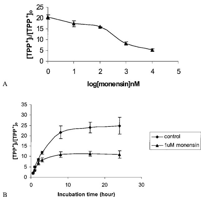
FIGURE 4. (A) Dose-dependent effects of monensin on TPP + uptake of rat lenses. Rat lenses were incubated in TC-199 medium with 10 \mu M TPP + and 10 nM to 10 \mu M monensin for 18 hours. (B) Accumulation of TPP + in rat lenses incubated in modified TC-199 medium with or without 1 \mu M monensin. TPP + (10 \mu M) was added to the media, and 1 \mu M monensin was added in one group at the beginning of the experiment. Data in (A) and (B) are presented as means \pm SE ( n \geq 4 ).
