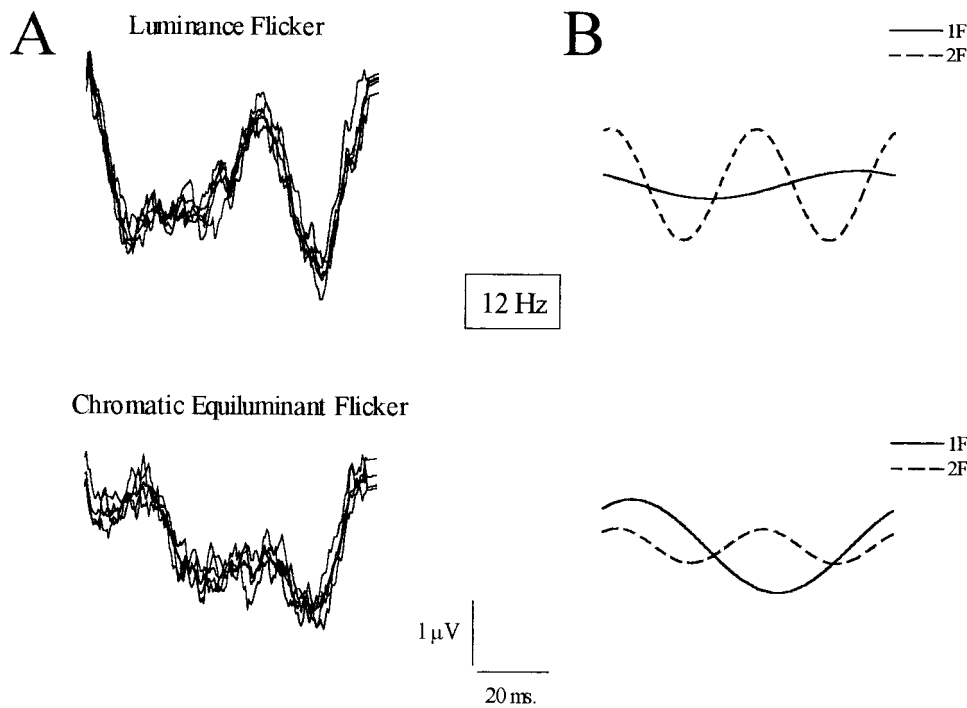
FIGURE 3. (A) Representative examples of flicker ERG recordings, obtained from one subject in response to luminance flicker and equiluminant chromatic flicker modulation at 12 Hz. Several blocks of responses are superimposed to demonstrate reproducibility. The sweep duration corresponds to one stimulus cycle (i.e., 83.3 ms). (B) 1F and 2F components of the grand average of the responses shown in (A).
