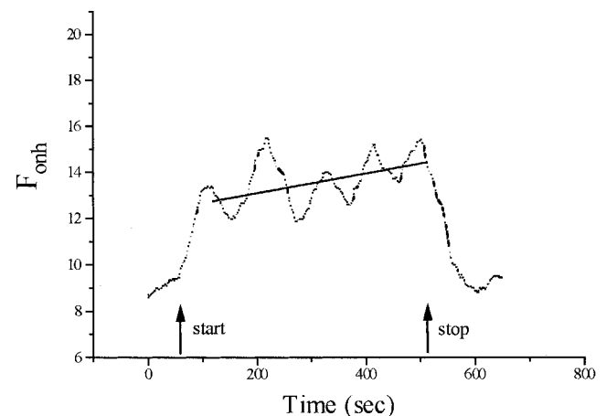
FIGURE 2. Smoothed recording of F_{0nh} (approximately 11 minutes) obtained from one subject in response to a 10-Hz, 13.5-lux G luminance flicker. Each data point represents an average during 2 seconds recording. A 10-point moving average procedure was used to smooth the data. Linear regression is fitted to the data points recorded between 125 and 525 seconds (start and stop, respectively), corresponding to the period of flicker stimulation.
