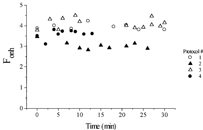
FIGURE 1. Baseline F_{0nh} obtained in one control subject, during the different recording sessions, plotted as a function of experimental time.
