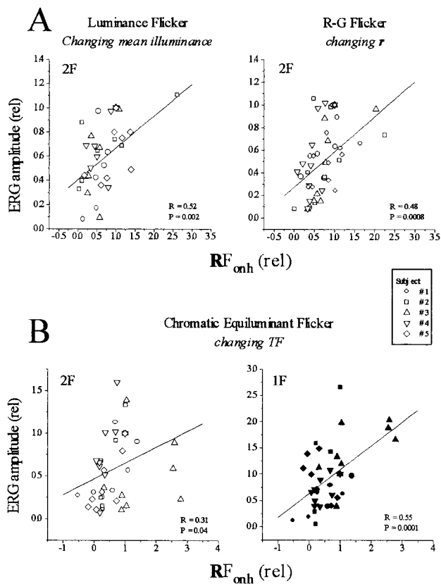
FIGURE 8. Mean RF_{oh} changes plotted as a function of corresponding ERG component amplitudes obtained in response to (A, left) G luminance flicker presented at different mean illuminance levels (protocol 2); (right) R-G hetero-chromatic flicker presented at different r (protocol 3); (B) R-G chromatic equiluminant flicker modulated at different Tf (protocol 4). All data recorded from the five subjects are shown in the scatterplots (each subject represented by a separate symbol). Correlation analyses performed only when RF_{oh} changes and ERG amplitudes showed similar functional shape. Coefficients ( r ) of the linear regressions to the data are reported in each scatterplot. Slopes of the regression lines are as follows: (A) Luminance flicker (protocol 2): 0.26; (A) R-G flicker (protocol 3): 0.31; (B) chromatic equiluminant flicker (protocol 4), RF_{oh} versus 2F: 0.18; (B) chromatic equiluminant flicker (protocol 4), RF_{oh} versus 1F: 0.45.
