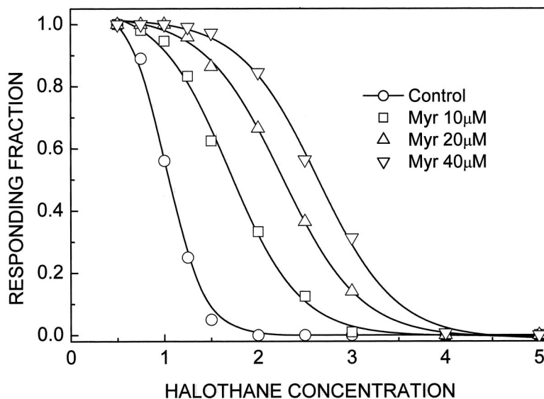
Fig. 1. Logistic plot of the effect of myristate on the halothane anesthesia. The concentrations of myristate are shown. The Y-axis contains information on the two unknown values ( ED_{50} and n ). Obtained best fit values are displayed in table 1.
