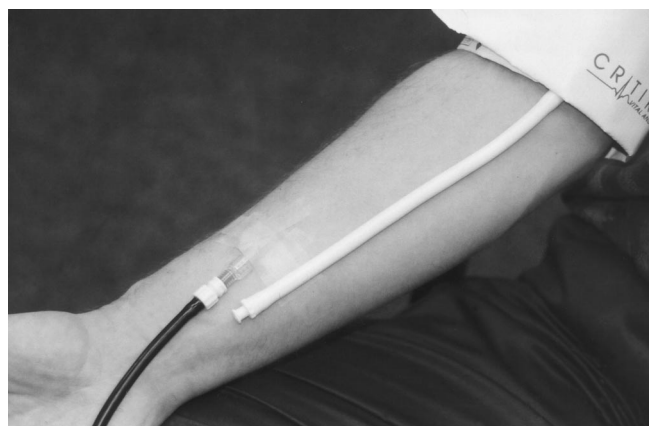
Fig. 2. Spacelabs Medical blood pressure inflation hose connected to an Alaris "heparin lock" 2000E instead of the Critikon Classic cuff 90426 connector.
