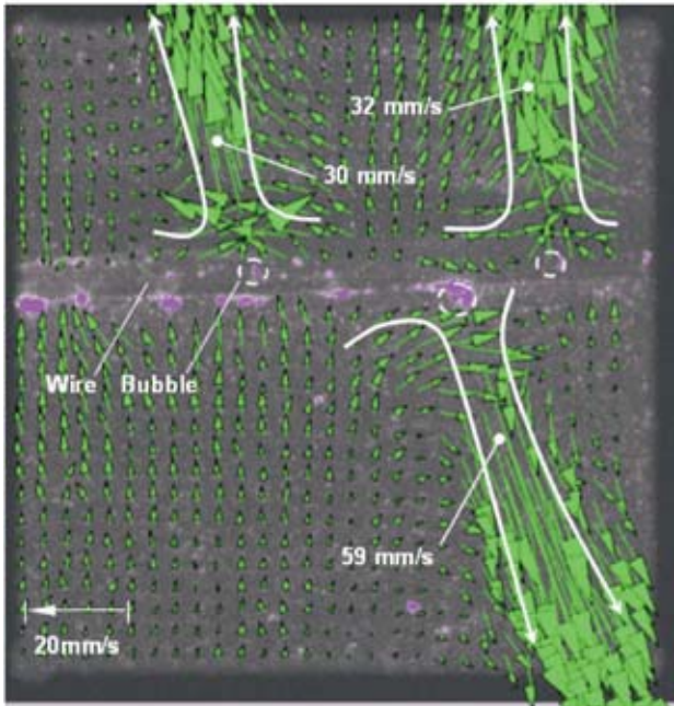
Velocities measured with PIV in bubble-top jets (water, T_{wire} = 378 K, T_{bulk} = 320 K)
