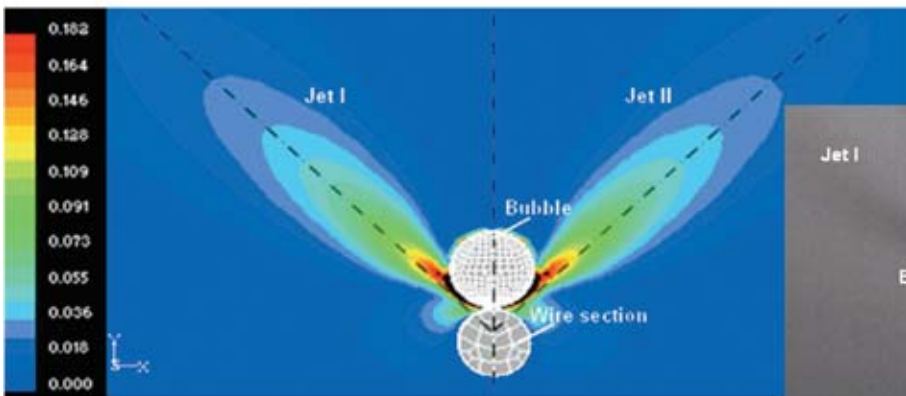
Simulation of butterfly-like structure of multi-jet flow: Velocity contours [m/s] (water, T_{wire} = 385 K, T_{bulk} = 335 K)
