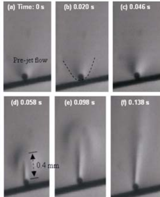
Two stages of the bubble-top jet formation process: Incipience (a)-(c), and Growth (d)-(f) (water, T_{wire} = 376 K, T_{bulk} = 330 K)
