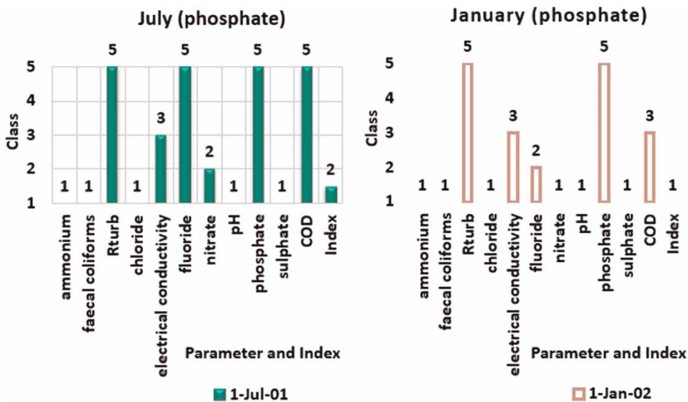
Figure 11 | Phosphate sensitivity analysis.
