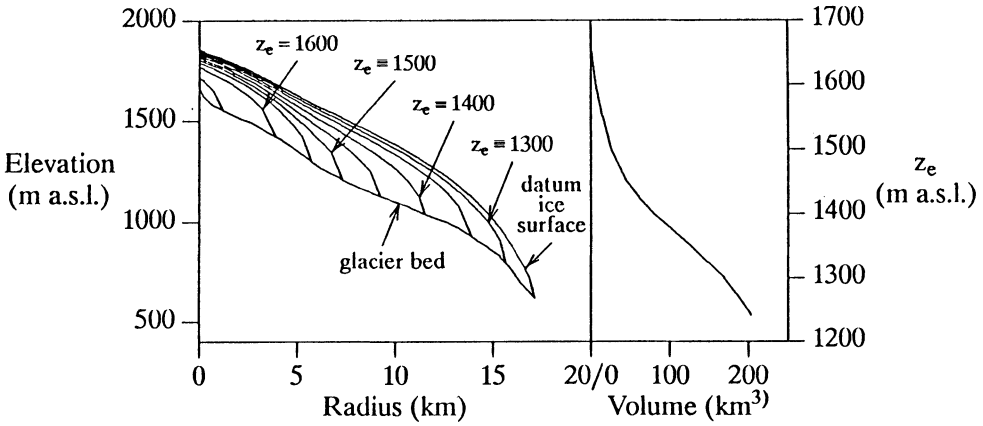
Fig. 3. Final steady state profiles for different equilibrium line altitudes z_e (left). The outermost profile is the datum ice surface profile corresponding to z_e = 1,240 m a.s.l. The inner profiles span the z_e range from 1,300 to 1,650 m a.s.l. with an increment of 50 m. The curve on the right shows the volume of the steady state profiles as a function of z_e .
