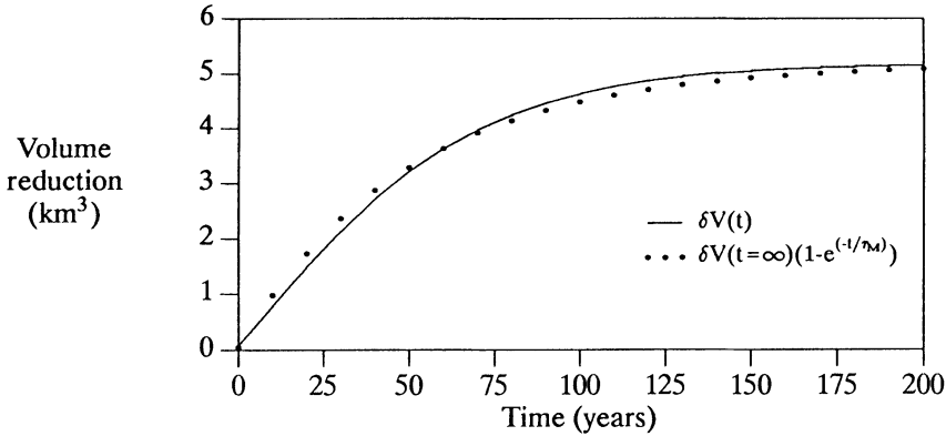
Fig. 5. Volume reduction as a function of time for a 10 m step change in z_e (solid curve). Mass balance – elevation feedback is taken into account. The dotted curve shows an exponential fit to the volume reduction with a response time \tau_M \equiv 50 years.
