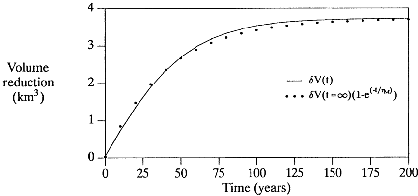
Fig. 4. Volume reduction as a function of time for a uniform step change in the mass balance of -0.075 m_{ice}a^{-1} which is equivalent to raising z_e by 10 m (solid curve). Mass balance – elevation feedback is not taken into account. The dotted curve shows an exponential fit to the volume reduction with a response time \tau_M \equiv 40 years.
