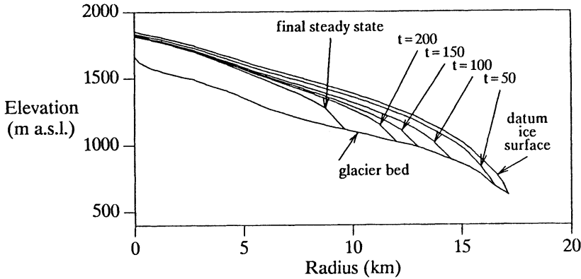
Fig. 6. Glacier profiles as a function of time with a time-dependent equilibrium line altitude z_e increasing linearly from 1,240 to 1,440 m a.s.l. during the initial 50 years of the model run and held fixed at 1,440 m a.s.l. after that. The outermost profile is the datum ice surface profile corresponding to z_e = 1,240 m a.s.l. The innermost profile is the final steady state profile corresponding to z_e = 1,440 m a.s.l. The intermediate profiles show the ice surface at t = 50, 100, 150 and 200 years.
