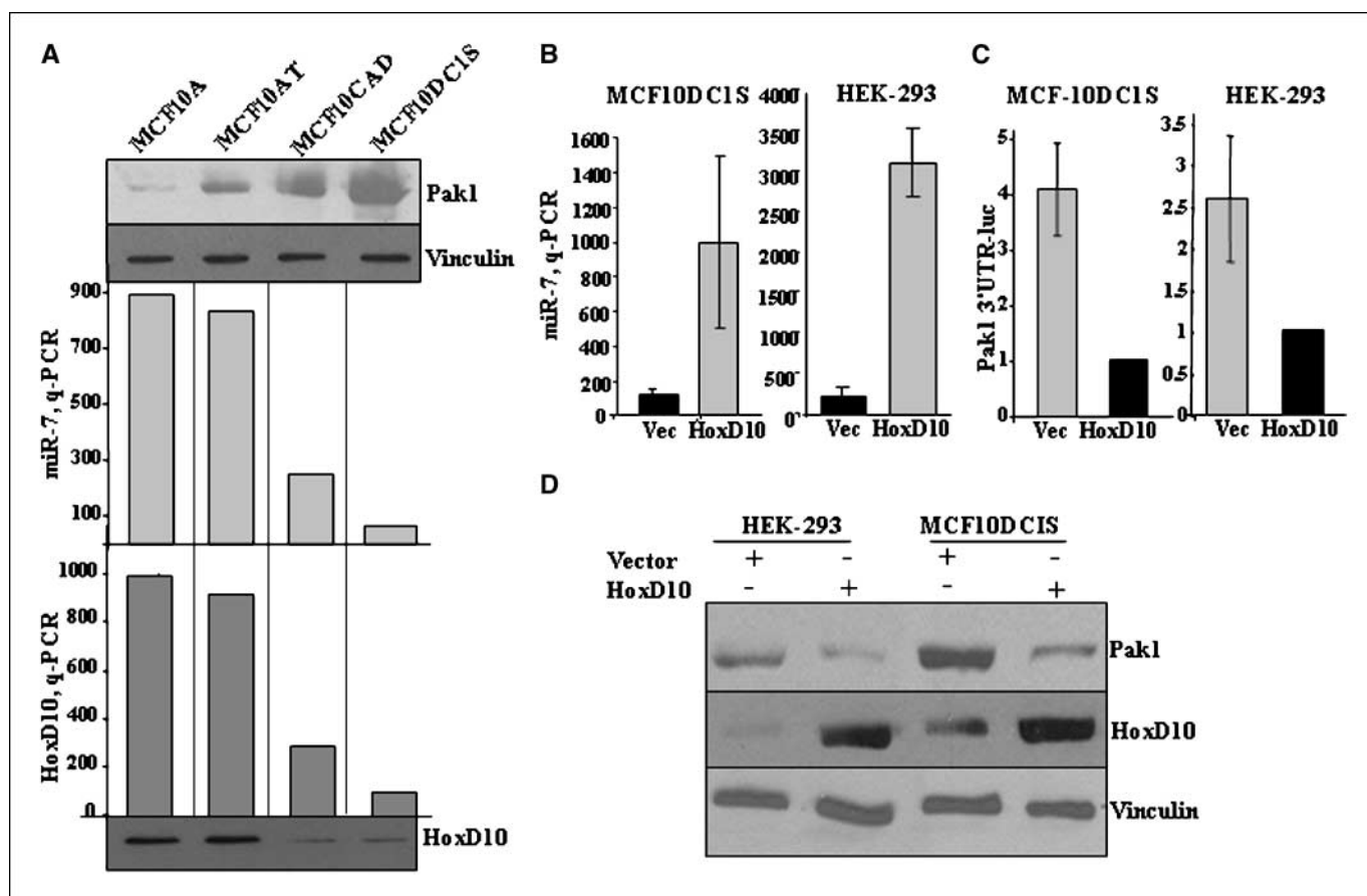
Figure 3. Dynamic correlation of Pak1, miR-7, and HoxD10 in the breast cancer progression model. A , Western blot analysis of Pak1 and HoxD10 and quantitative PCR analysis of the endogenous miR-7 and HoxD10 in the MCF10A model system. B , effect of HoxD10 expression on the levels of miR-7 in MCF-10-DCIS and HEK-293 cells. Columns, mean of three experiments; bars, SD. C , normalized Pak1 3'-UTR-luc activity in MCF10DCIS and HEK-293 cells transfected with HoxD10 or control vector. Columns, mean of three experiments; bars, SD. D , Western blot analysis of Pak1 and vinculin in MCF10-DCIS and HEK-293 cells transfected with HoxD10 or control vector.
