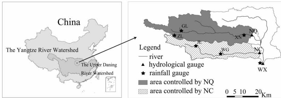
Figure 1 | Location map of the study watershed and the three hydrological gauges.
