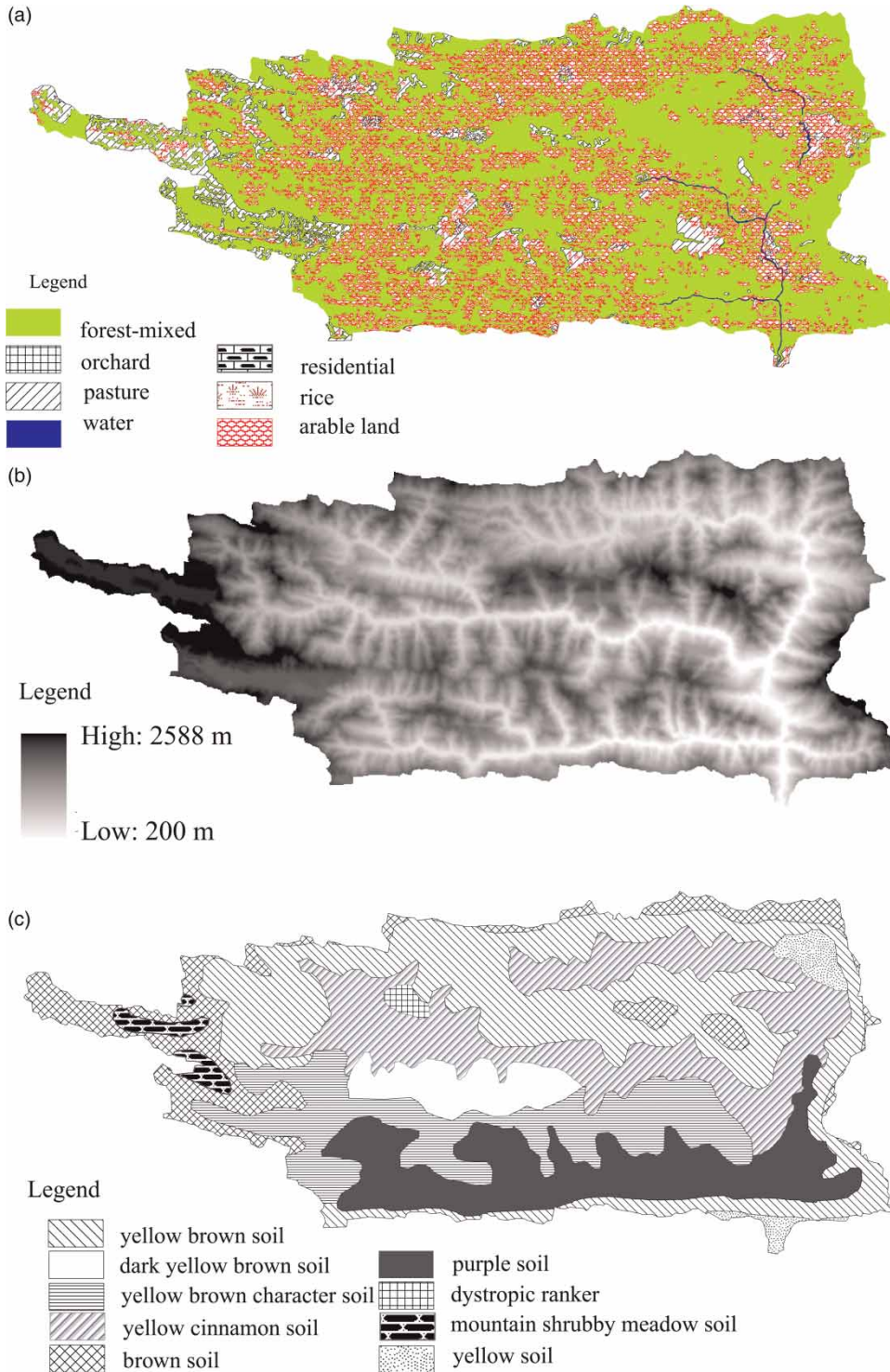
Figure 3 | Spatial characteristics of the Upper Daning River Watershed. (a) Land use distribution; (b) Topography distribution; (c) Soil type distribution.
