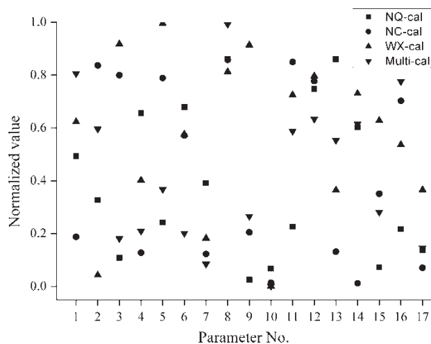
Figure 4 | Normalized parameters obtained by four schemes (the parameter no. is listed in Table 2).
