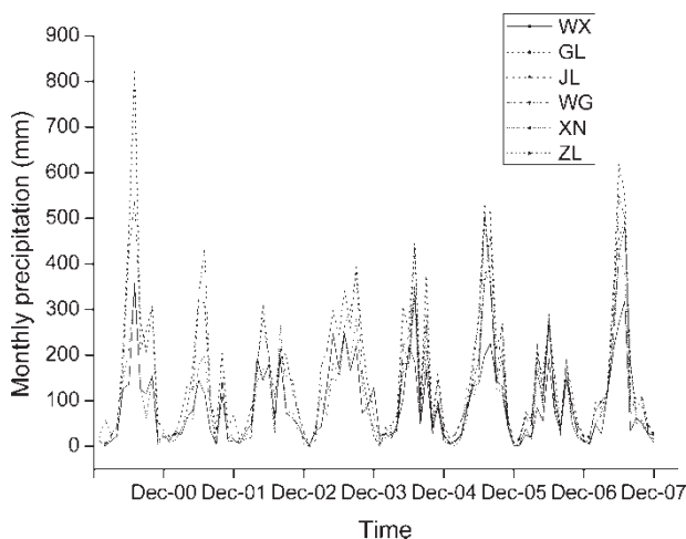
Figure 2 | Monthly precipitation of the rainfall gauges for 2000–2007.
