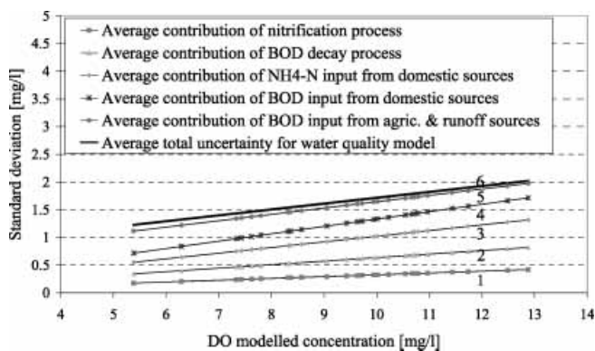
Figure 14 | Average total uncertainty for the DO model, together with the average uncertainty contribution of (1) nitrification process, (2) BOD decay process, (3) \text{NH}_4\text{-N} input from domestic sources, (4) BOD input from domestic sources, (5) BOD input from agricultural and runoff sources and (6) model structure and measurements.
