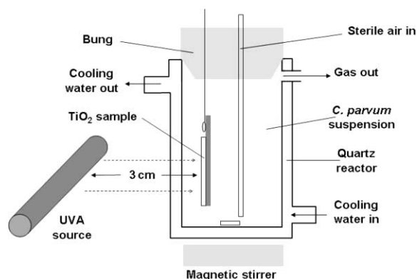
Figure 1 | Photocatalytic reactor.
