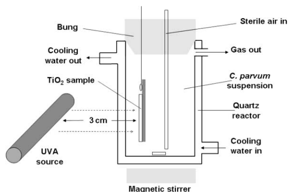
Figure 1 | Photocatalytic reactor.
