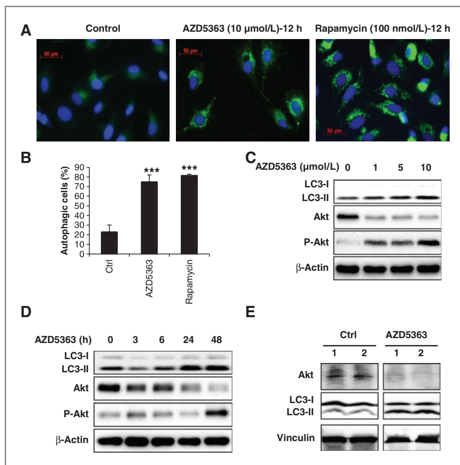
Figure 3. AZD5363 induces autophagy in vitro and in vivo . A , PC-3 cells were treated with 10 μmol/L AZD5363 or with 100 nmol/L rapamycin for 12 hours as positive control of autophagy induction. LC3 detected by immunostaining was analyzed and compared with control. Puncta represent autophagosome formation. B , quantification of puncta from A representing proportion of autophagic cells. PC-3 cells were treated with AZD5363 at indicated doses for 48 hours ( C ) or with 10 μmol/L for indicated time points ( D ). Protein extracts were analyzed by Western blotting for LC3-I, LC3-II, Akt, and p-Akt. β-Actin was used as the loading control. E , male C57-BL-6J black mice were treated with vehicle control or AZD5363 (100 mg/kg) for 6 hours. The Akt, LC3-I, and LC3-II levels were examined in the whole protein lysates prepared from heart tissues. Vinculin was used as the loading control.
