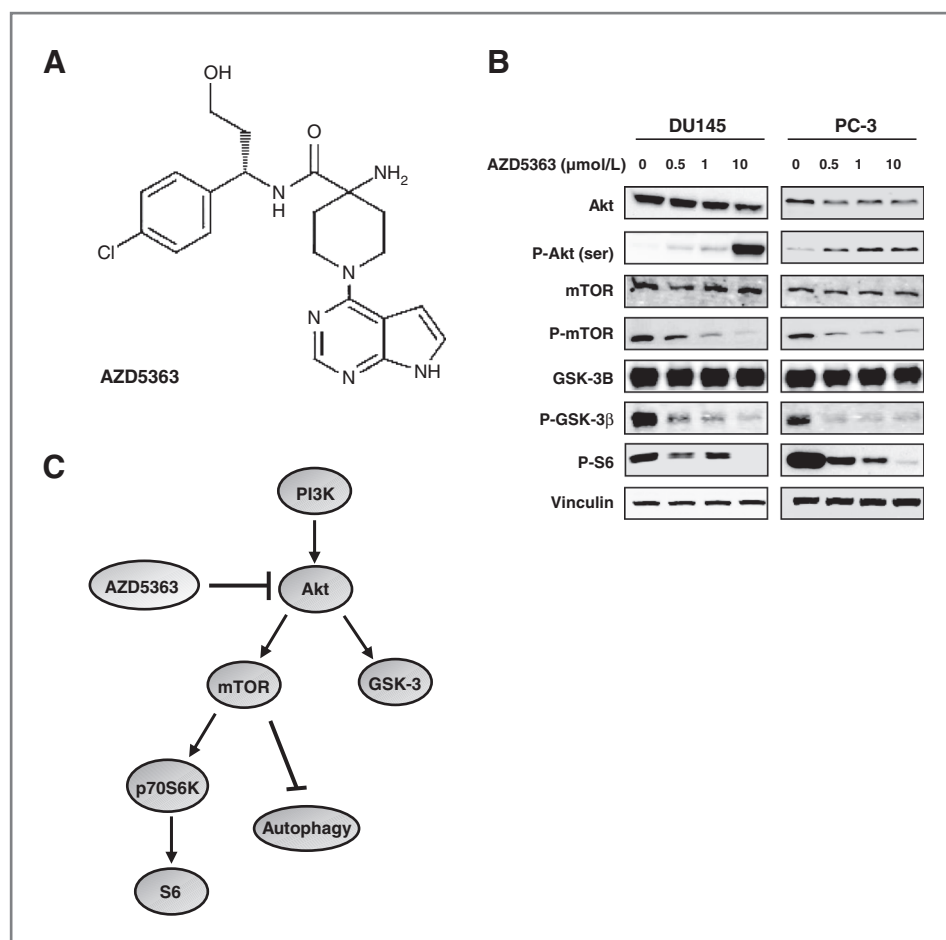
Figure 1. AZD5363 inhibits PI3K/Akt/mTOR pathway. A, chemical structure of AZD5363. B, PC-3 and DU145 cells were treated with AZD5363 at indicated doses for 48 hours. Cell lysates were analyzed by immunoblotting with antibodies as indicated. C, a model depicting Akt-mediated signal pathway, also involved in the suppression of autophagy via mTOR activation.
