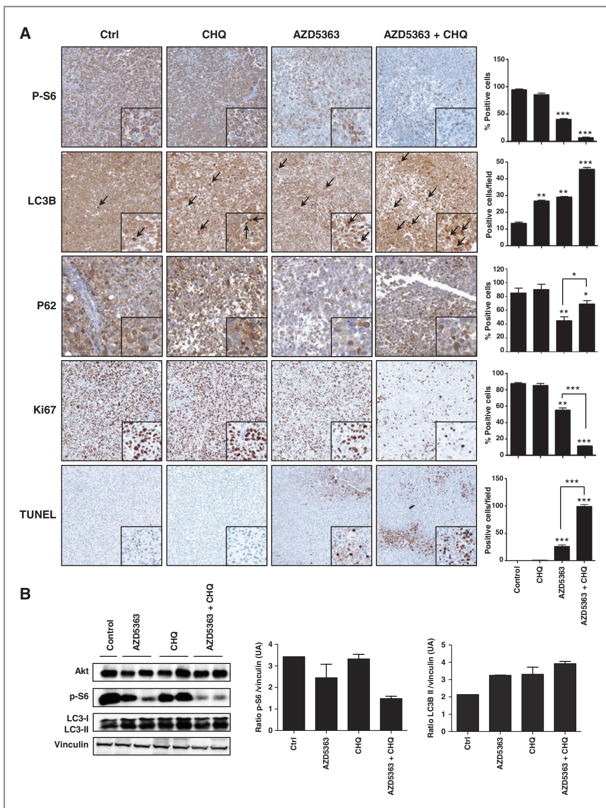
Figure 6. AZD5363 and chloroquine cause apoptosis in xenograft model. A , tumors were collected after sacrifice and p-S6, Ki67, LC3, and terminal deoxynucleotidyl transferase–mediated dUTP nick end labeling (TUNEL) were evaluated by immunohistochemical analysis (original magnification, \times 200 ). Specimens were scored and estimated in positive cells per field or in percentage of positive cells. B , total proteins were extracted from the xenograft tumors and Akt, p-S6, LC3-I, and LC3-II were analyzed by Western blotting. The relative levels were normalized with vinculin and estimated in densitometric units \pm SEM; ***, P < 0.001 ; **, P < 0.01 ; *, P < 0.05 .
