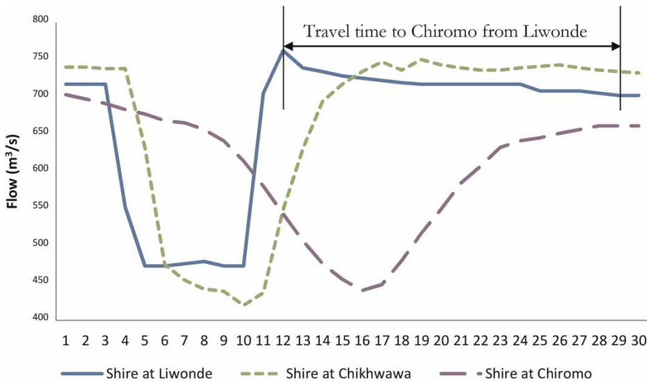
Figure 6 | Hydrographs of Shire River flows at Liwonde, Chikhwawa and Chiromo following a test run at Liwonde barrage upstream in November 1981. Source: MoIWD.
