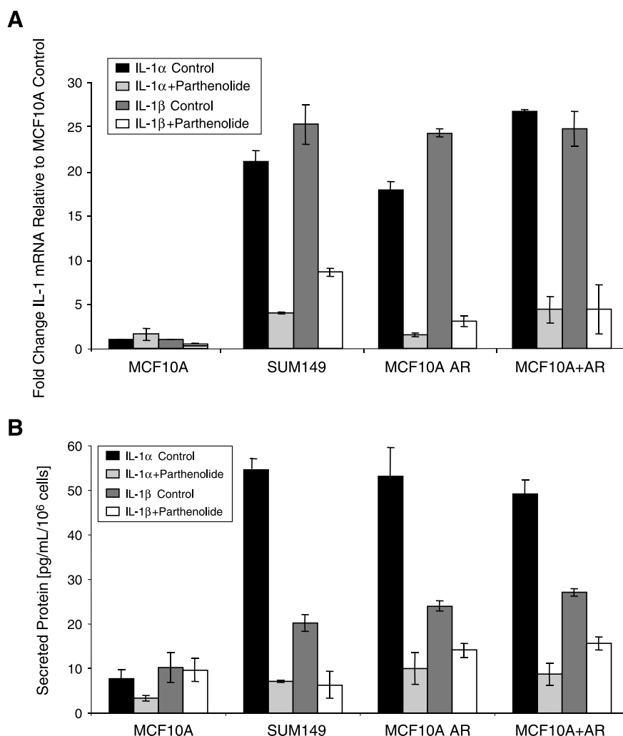
FIGURE 4. AR-stimulated EGFR increases IL-1 mRNA and secretion in an NF- \kappa B-dependent manner. IL-1 \alpha and IL-1 \beta mRNA expression (A) and secreted protein levels (B) were measured in MCF10A AR, MCF10A+AR, SUM149, and MCF10A cells by quantitative, real-time PCR and ELISA, respectively. EGFR activation was inhibited by 10 \mu mol/L of the NF- \kappa B inhibitor parthenolide. Columns, means of three independent experiments; bars, SD. Fold change relative to MCF10A control.
