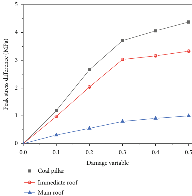
FIGURE 13: Variation rule of peak stress difference under different damage variables.
